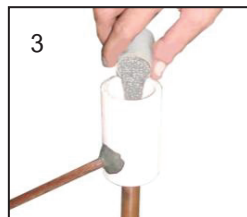
3 Dump OneTime Weld metal in mold.
