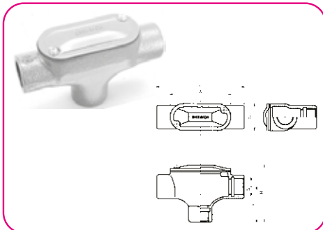
Flame-Proof Explosion Protected Type ISET TEE (back)
