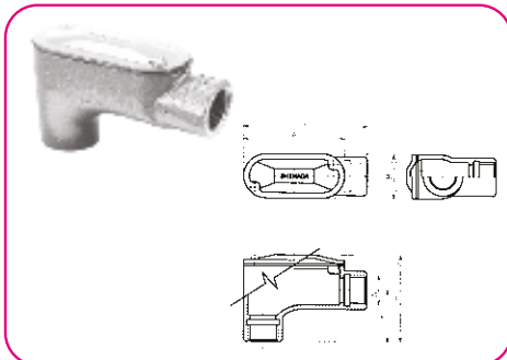
Flame-Proof Explosion Protected Type ISEB (LB) Elbow (back)
