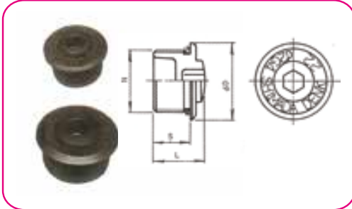
Flame-proof Explosion-Protected Blind Plugs (d2G4) Type SBP Blind Plugs
