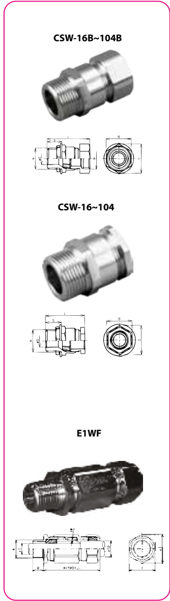
Industrial Type (Outdoor) Cable Gland Type CSW-B Male Thread x Female Thread Type
