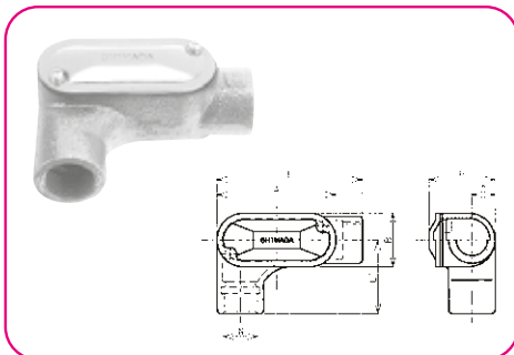
Flame-Proof Explosion Protected Type ISER Elbow (Right)
